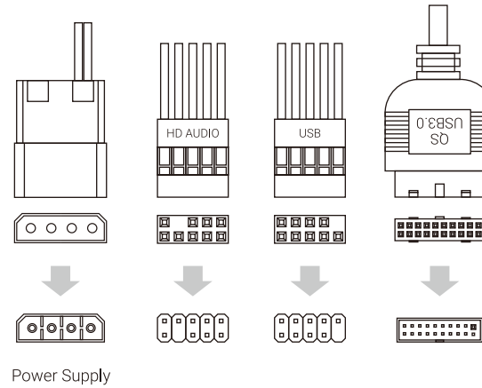
Power Supply
