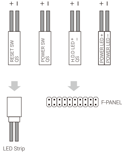
LED Strip
